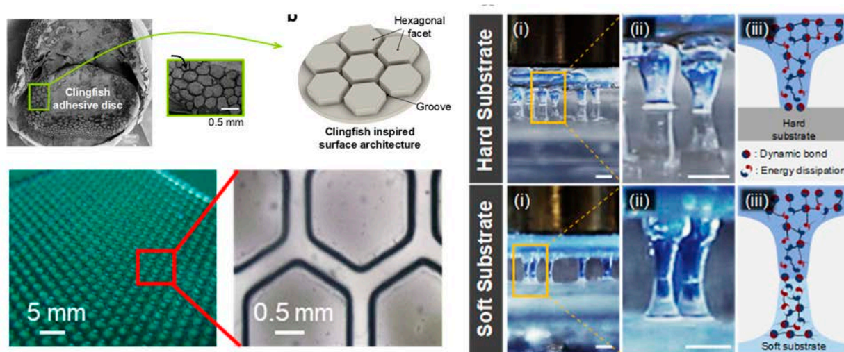
Figure A-9. Functions through macroscopic geometry and morphology control. (b) Photograph and optical microscopy image of the surface structures on a polyampholyte (PA) hydrogel, and photograph of patterned gels during debonding from a glass plate under water. Rao et al., Advanced Materials , 2018.
